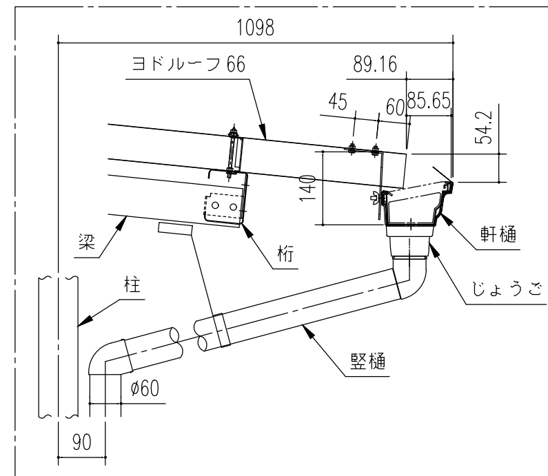
“A”部詳細 (S = 1/10)
