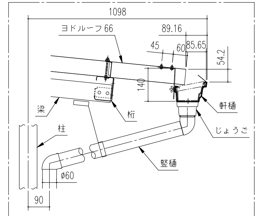
“A”部詳細 (S = 1/10)
